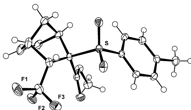
Figure 1. X-ray structure of 15 (50% probability level).
