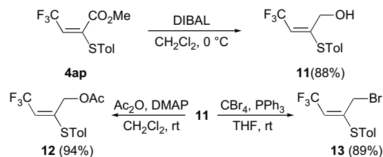
Scheme 8. Transformation of 4ap .
