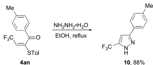
Scheme 6. Synthesis of pyrazole 10 .
