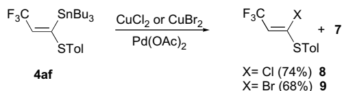
Scheme 5. Halogenation of 4af with CuCl 2 or CuBr 2 .
