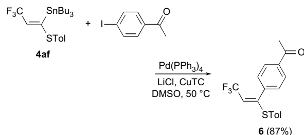
Scheme 4. Cross-coupling reaction of 4af with 4'-iodoacetophenone.
