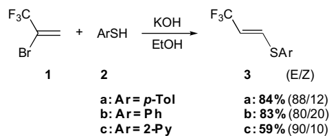
Scheme 1. Preparation of \beta -(trifluoromethyl)vinyl sulfide 3 .
