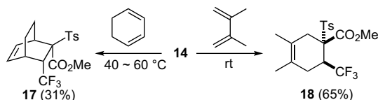
Scheme 11. Diels–Alder reaction of 14 with two dienes.
