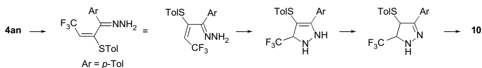
Scheme 7. Plausible mechanism for the formation of 10 .
